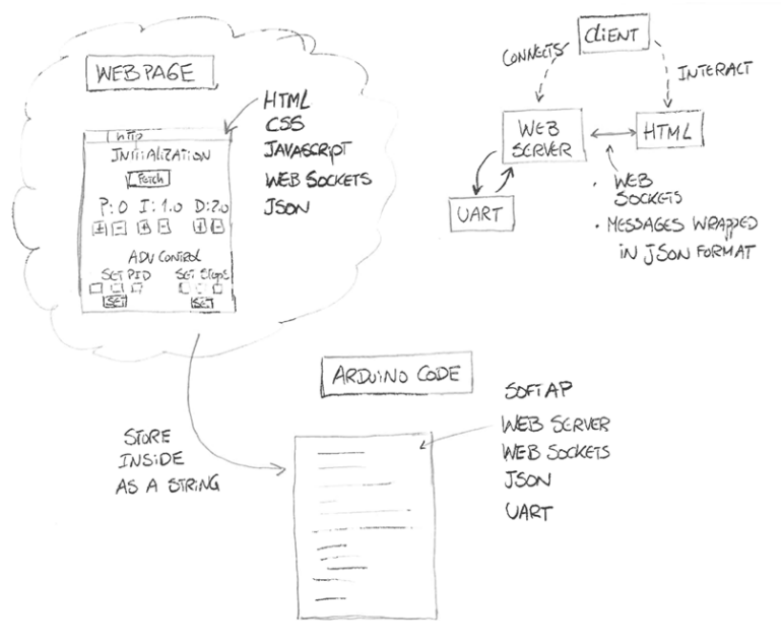
Figure 2: Planned ESP8266 web interface and UART communication structure.
